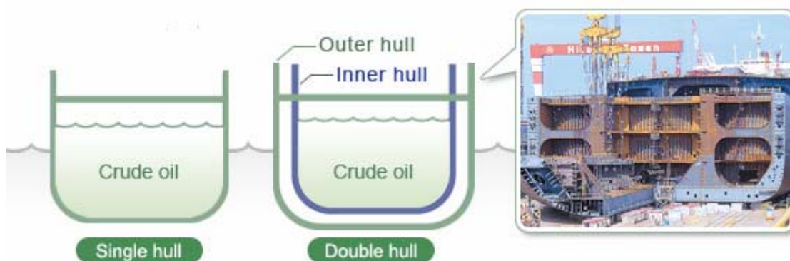
Double Hull Ship;
