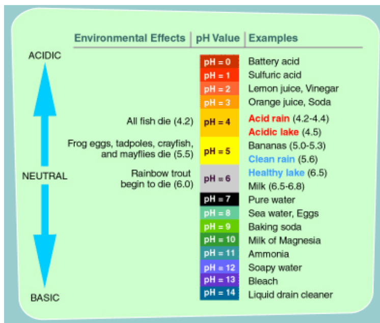
pH Value of Common Household Items and the Environmental Effects pH on Water; http://www.epa.gov/acidrain/education/site_students/phscale.html
