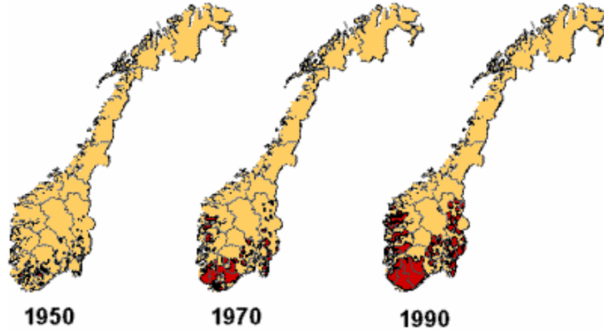
Lost or Damaged Fish Stocks Due to Acid Rain
